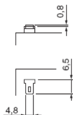
■ Type 1 Faston 4.8
