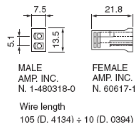
■ Type 6 Wire and connector
