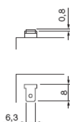
■ Type 2 Faston 6.3
